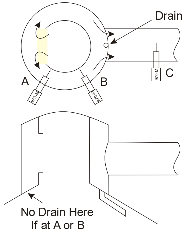
Figure 5: Locating the Sensor Element on Pans with Cast Iron Domes and Separators
