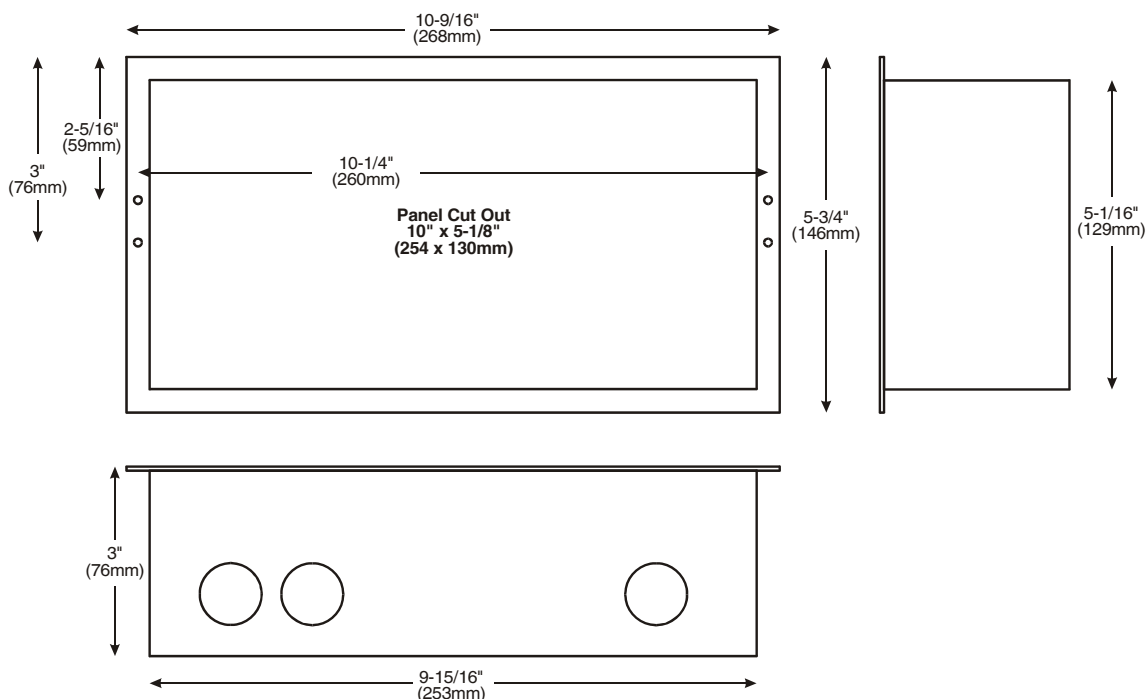
Figure 2: Monitor Mounting Dimensions
