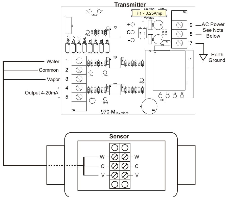
Figure 4: Connecting Measuring Element and Monitor
