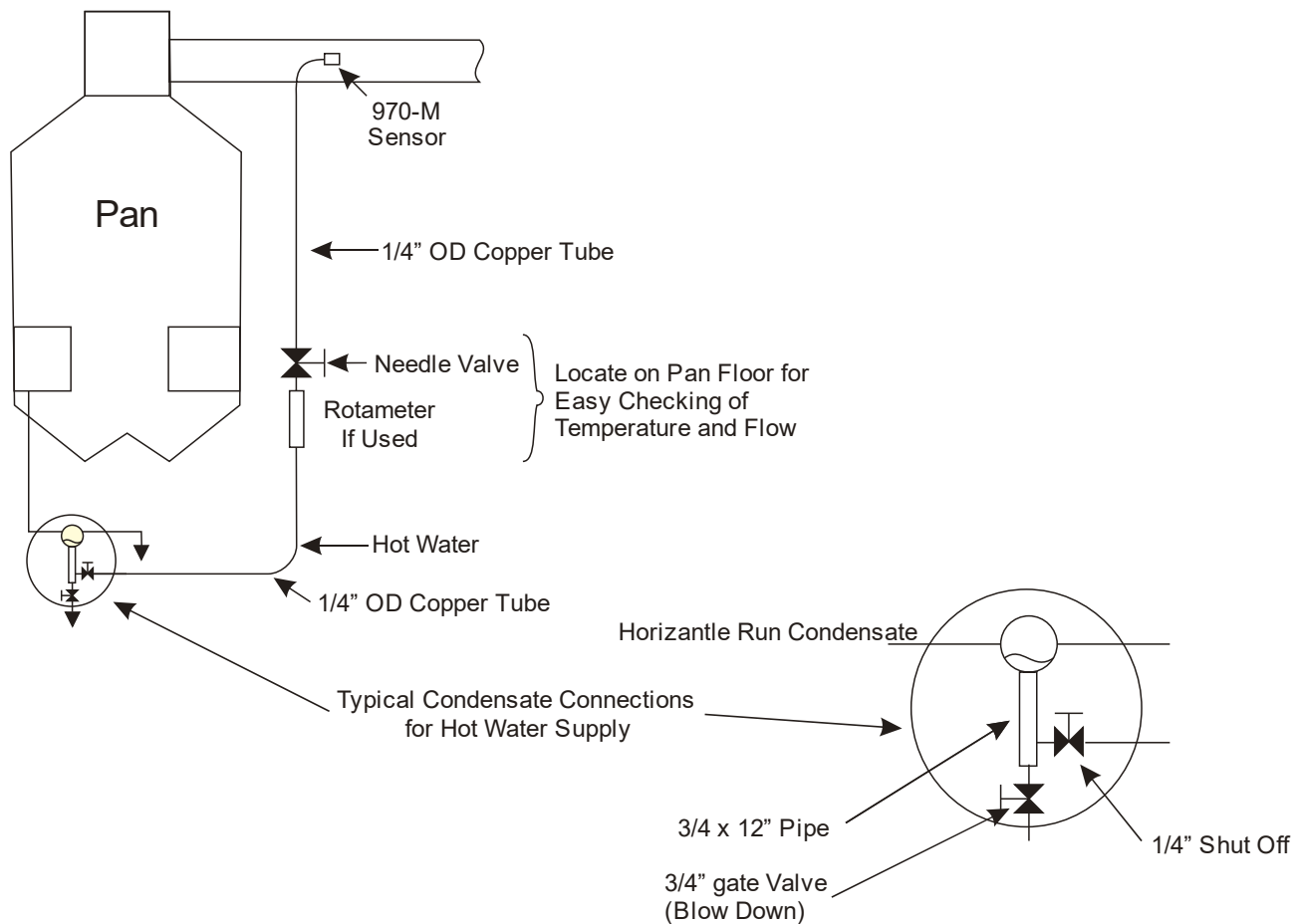
Figure 1: Hot Water Supply
